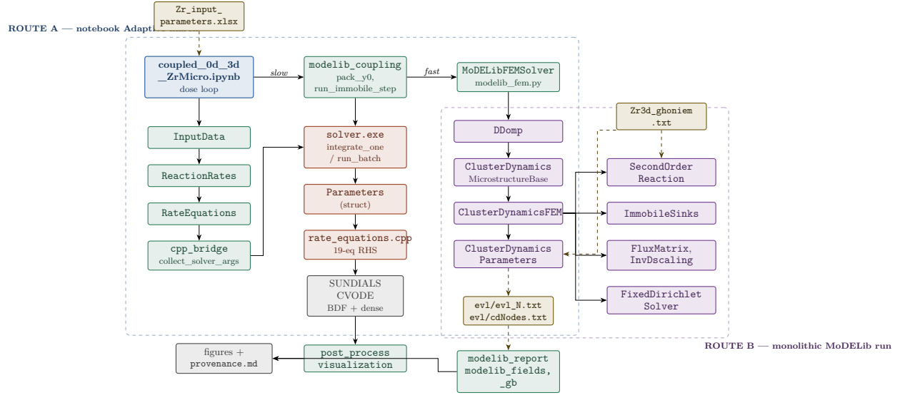
Figure 1: Component call graph. Solid arrows are calls, dashed arrows are file input/output. Blue: orchestrating notebook; green: ZrMicro Python; red: ZrMicro C++; purple: MoDELlib3 C++; ochre: files on disk; gray: products. Route A drives the fast mobile solve through MoDELlib3 and the slow immobile march through the ZrMicro integrator; Route B runs both inside MoDELlib3. The two routes share the material definitions and the post-processing layer.
